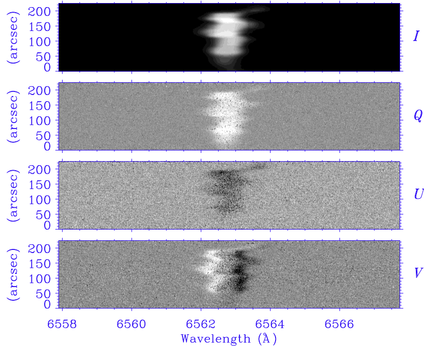
Fig. 6. Example of full Stokes spectro-polarimetric recording of an erupting prominence in H_{\alpha} .
