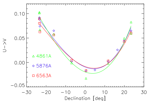
Figure 2. Measurement of the U \rightarrow V crosstalk as a function of declination for H\alpha , He-D3 and H\beta . To obtain this measurement the linear polarizer is rotated by 45^\circ with respect to the geographical equator.
