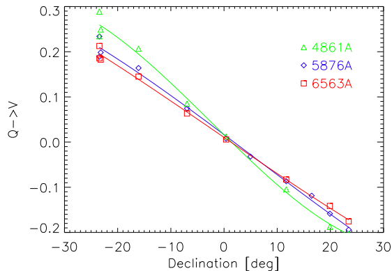
Figure 1. Measurement of the Q \rightarrow V crosstalk as a function of declination for H\alpha , He-D3 and H\beta . To obtain this measurement a linear polarizer is placed before the entrance window of the telescope with the polarization axis parallel to the geographic equator which is our choice here for the positive direction of Stokes Q .
