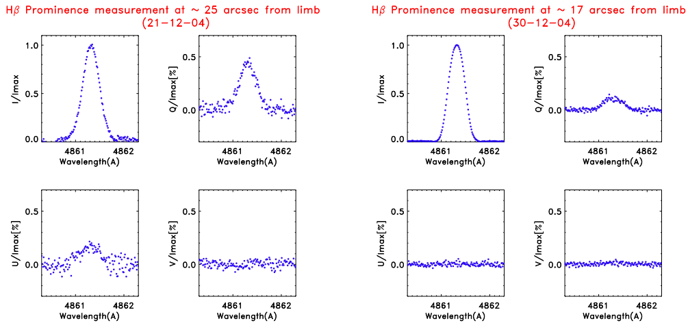
Figure 5. Two examples of H\beta recordings of Stokes profiles.
