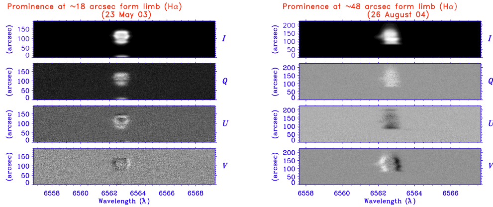
Figure 2. Two examples of H\alpha measurements.
