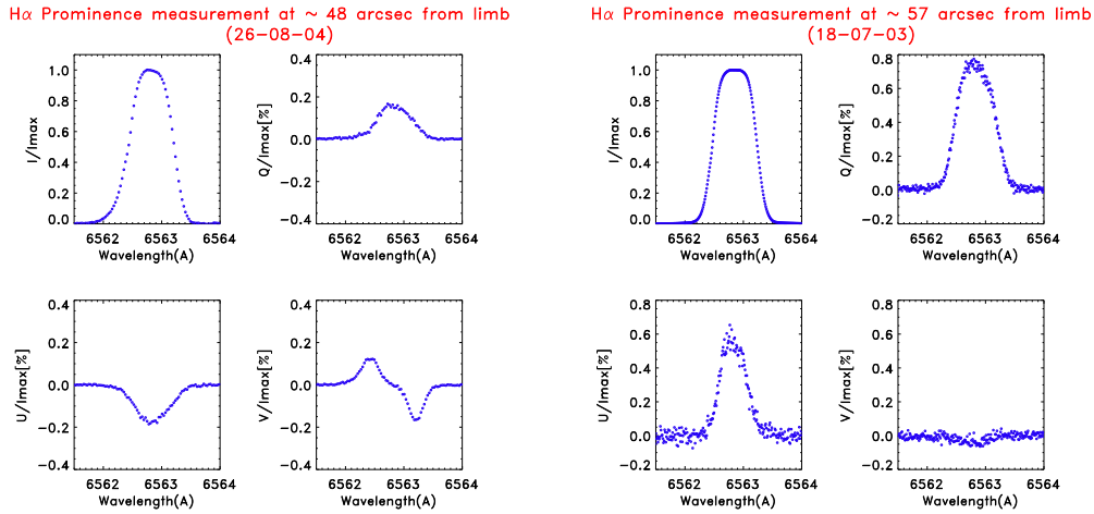
Figure 3. Two examples of H\alpha Stokes profiles. In the first example left we see a typical antisymmetric Zeeman like structure in Stokes V . The second example right is the only case where we find a symmetric structure in Stokes V . The amplitude in this case is only a few 10^{-4} .
