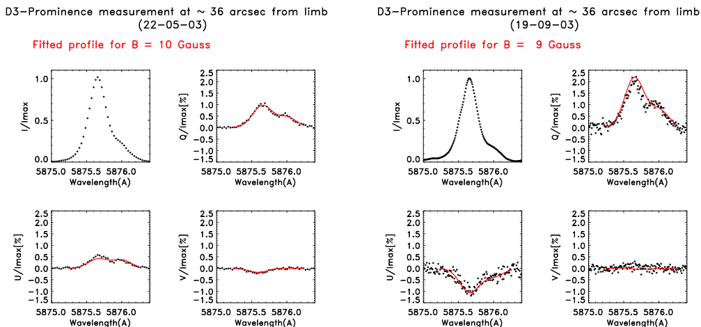
Figure 1. Two examples of He-D 3 Stokes profiles obtained from prominence observations with fitted theoretical profiles (continuous line).
