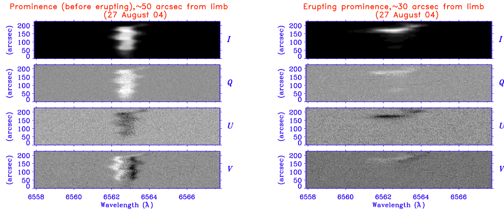
Figure 4. Example of H\alpha measurements. Left : Prominence before erupting Right : Prominence during eruption
